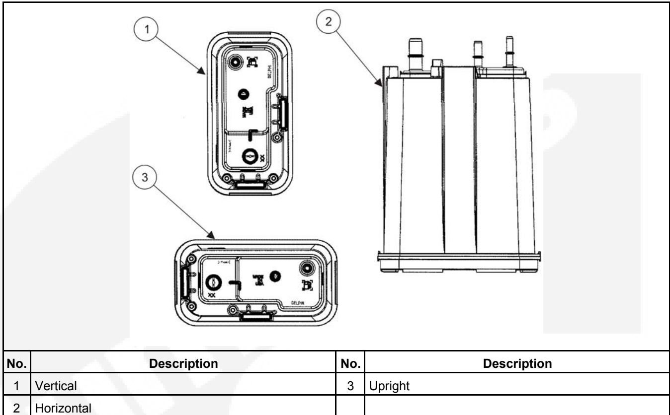
FIGURE 12. ACCEPTABLE CANISTER MOUNTING ORIENTATIONS
