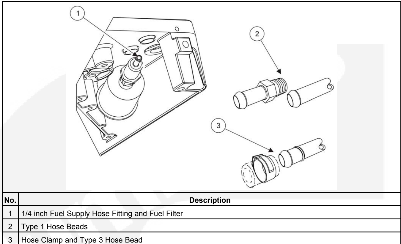
FIGURE 9. GASOLINE MOTORIZED FUEL CONNECTION
