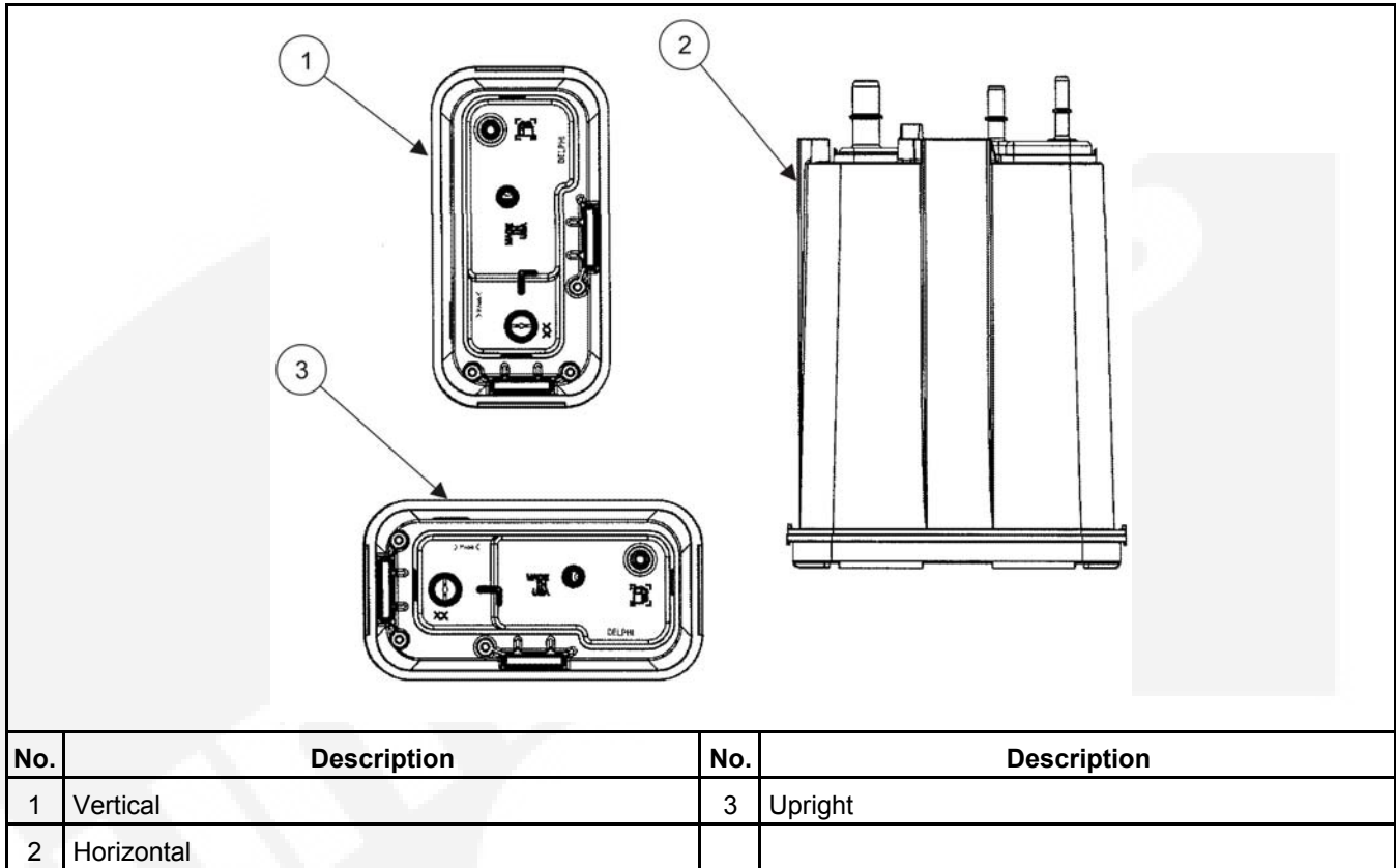
FIGURE 14. ACCEPTABLE CANISTER MOUNTING ORIENTATIONS
