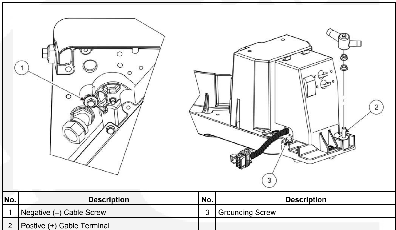
FIGURE 26. BATTERY CABLE CONNECTIONS
