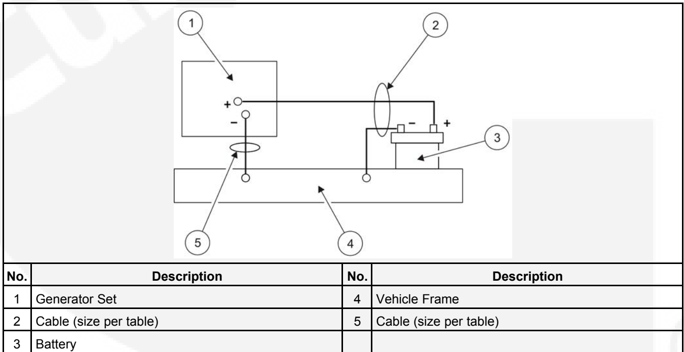
FIGURE 25. VEHICLE FRAME AS PATH FROM BATTERY NEGATIVE (-) TERMINAL
