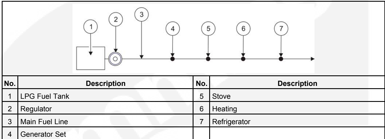
FIGURE 18. LPG FUEL LINE APPLIANCE CONNECTIONS (2.5 THROUGH 5.5 KW LPG SYSTEMS)
