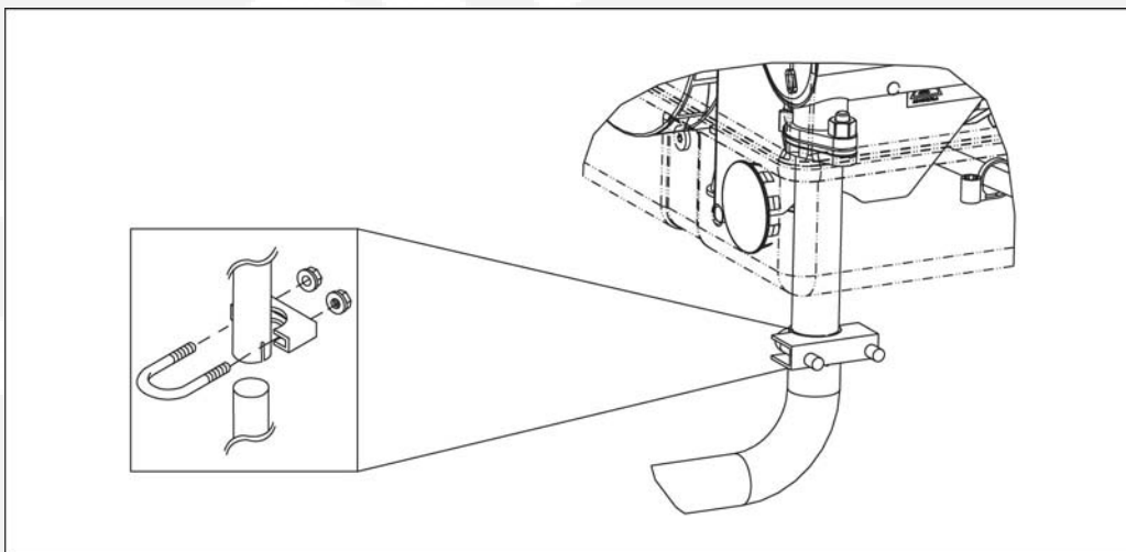
FIGURE 6. EXHAUST TAILPIPE CONNECTIONS
