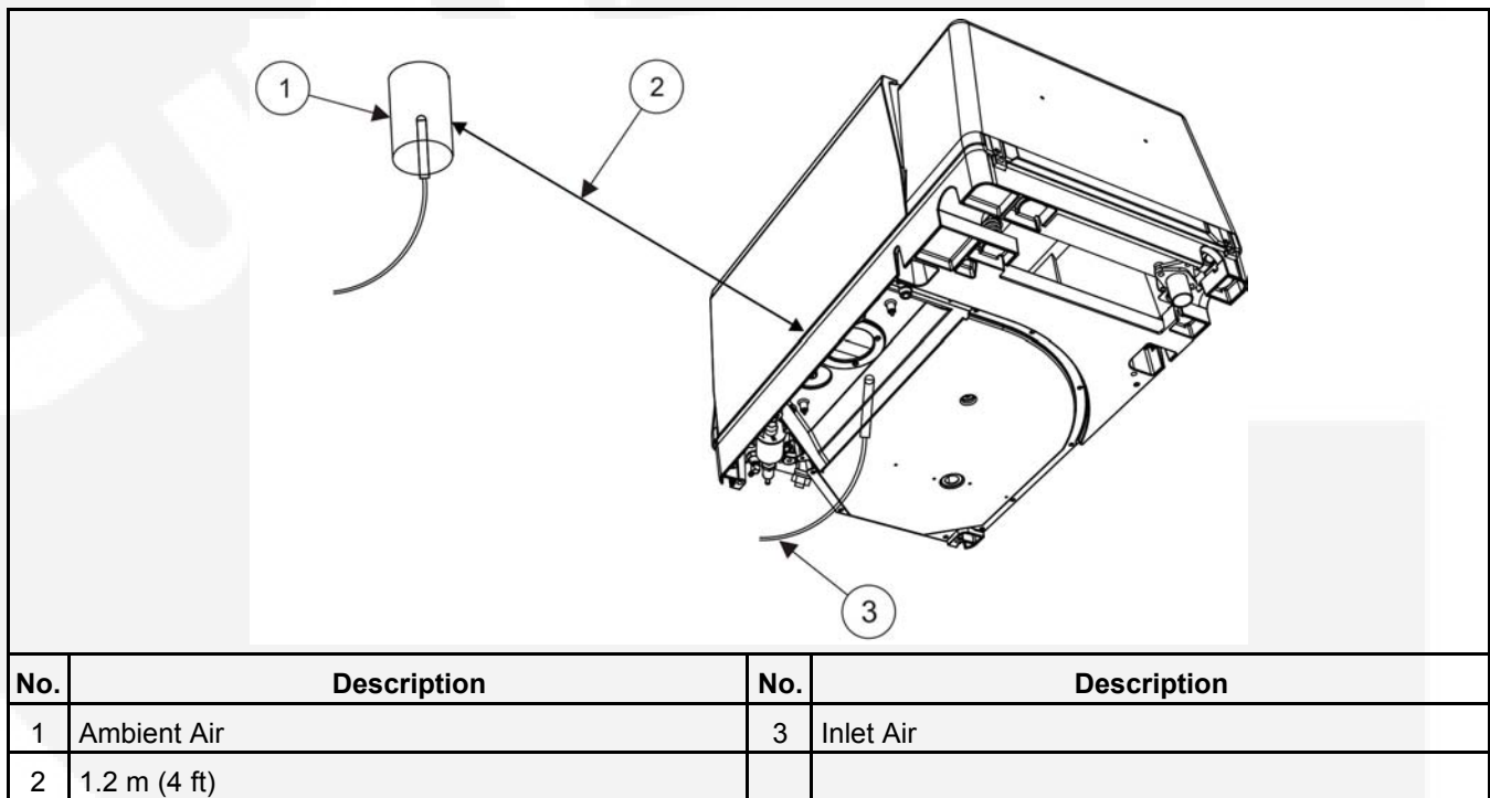
FIGURE 27. THERMOCOUPLE LOCATIONS FOR HOT AIR RECIRCULATION TEST
