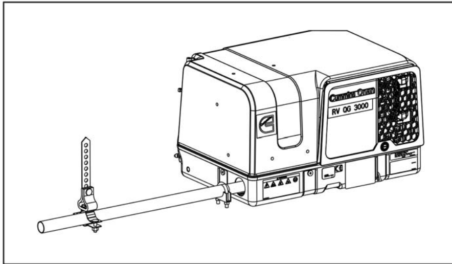
FIGURE 5. TYPICAL TAILPIPE INSTALLATION (SIDE OF UNIT)
