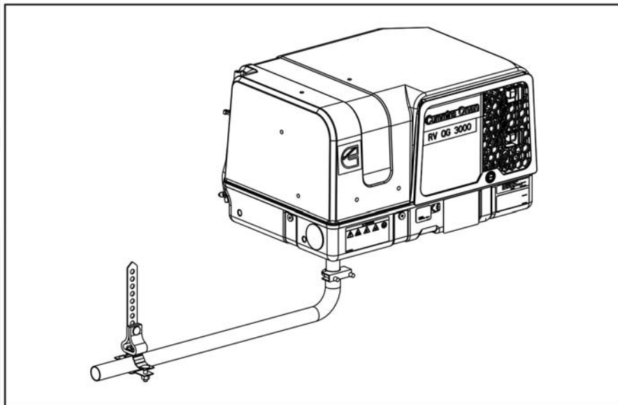
FIGURE 4. TYPICAL TAILPIPE INSTALLATION (BOTTOM OF UNIT)
